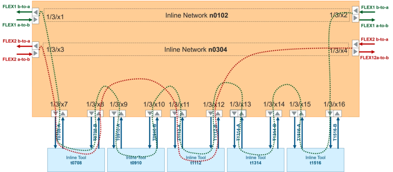
Figure 14 Example 6 Inline Tool Sharing by Multiple Inline Flows
