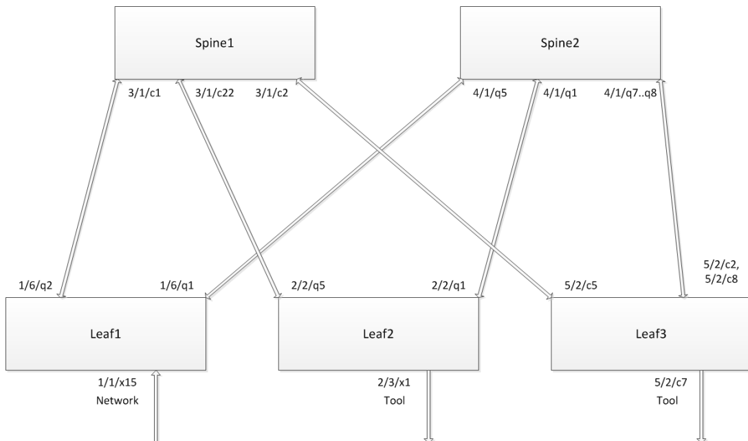
Figure 27 Configuration Leaf Spine Topology
